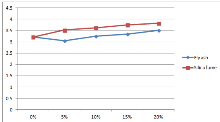
Figure A6. Comparison of 28 days split tensile strength of SCC with fly ash and silica fume
