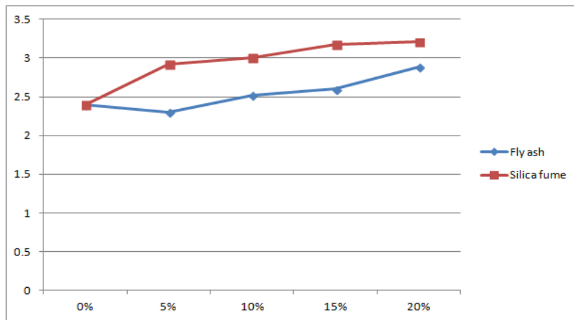
Figure A5. Comparison of 7 days split tensile strength of SCC with fly ash and silica fume
