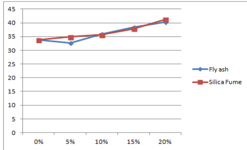
Figure A4. Comparison of 28 days compression strength of SCC with fly ash and silica fume
