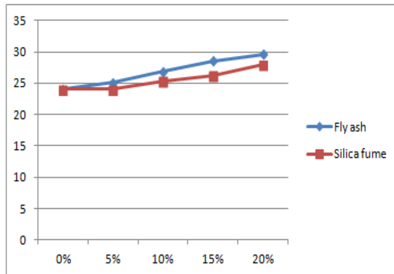
Figure A3. Comparison of 7 days compression strength of SCC with fly ash and silica fume
